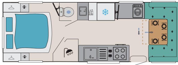
CRV 691 BODY LENGTH: 6.9m (22.6 ft)
