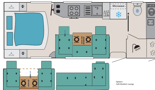
CRV 651 BODY LENGTH: 6.5m (21.4 ft)
