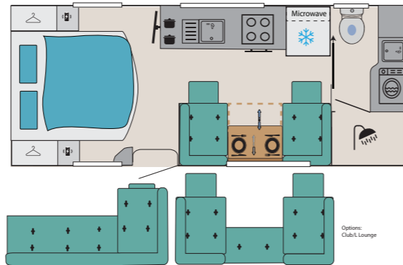
CRV 571 BODY LENGTH: 5.7m (18.7 ft)
